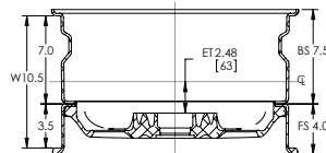
SECTION F-F
