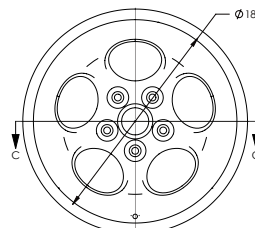
③ PHONE DIAL, 18 X 9 ET57 P/N 928-PD-18X9-ET57-944-REAR
