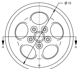
① PHONE DIAL, 18 X 8 ET57 P/N 928-PD-18X8-ET57-944-FNT
