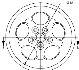
② PHONE DIAL, 18 X 9 ET69 P/N 928-PD-18X9-ET69-928-FNT
