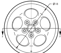
⑥ PHONE DIAL, 18 X 10.5 ET63 P/N 928-PD-18X10.5-ET63-928-REAR
